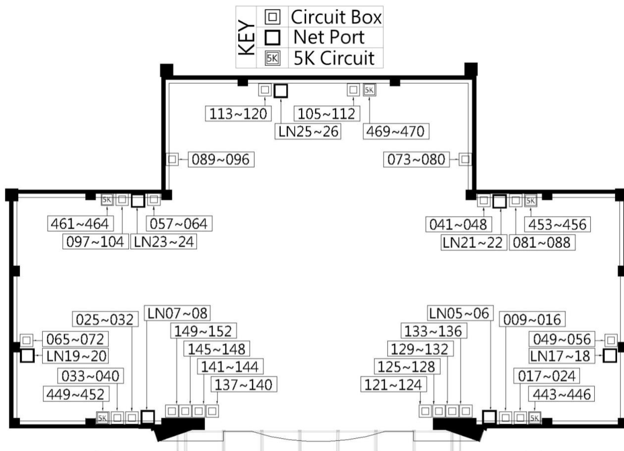
Figure 2.3.1- Stage Area Circuit Layout
