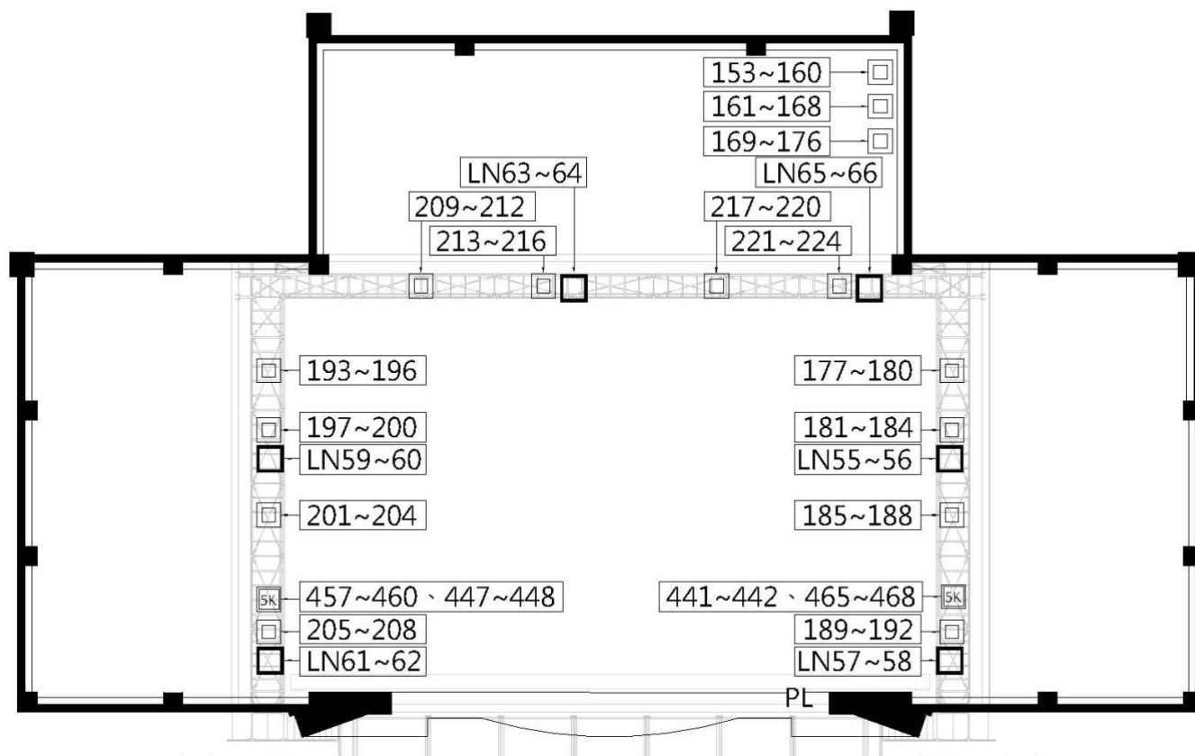
Figure 2.3.2- Gallery Circuit Layout
