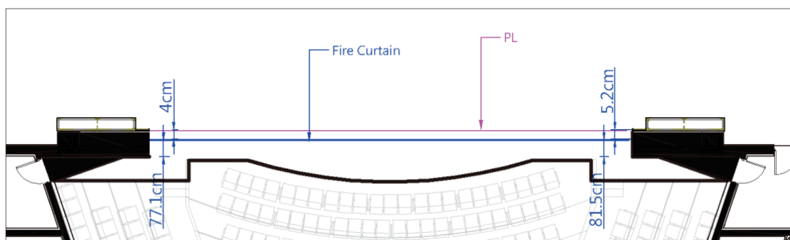
Figure 1.5.2- Fire Curtain
