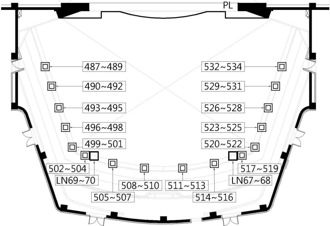
Figure 2.3.6- Balcony Rail Circuit Layout
